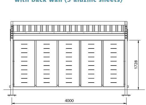
Triangle single sided starter section with back wall (5 aluzinc sheets)
